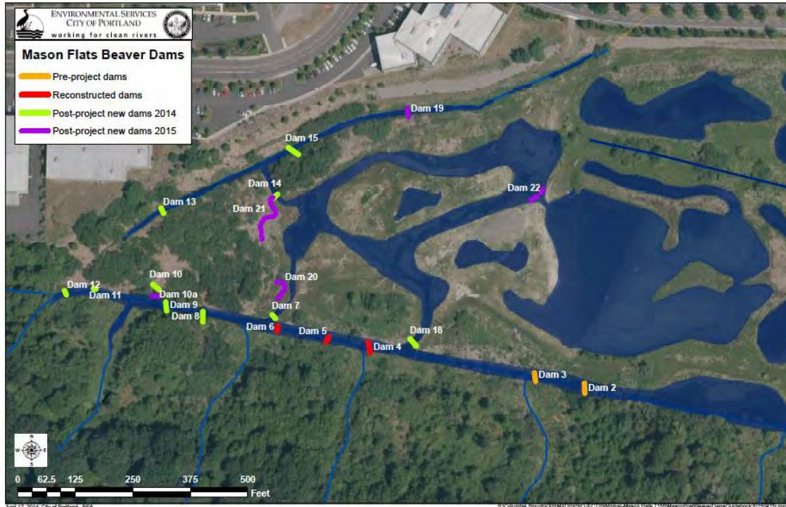
Figure 53: 2015 aerial photo of the site showing locations of old, reconstructed, and newly constructed beaver dams. Figure courtesy of City of Portland, Environmental Services.
