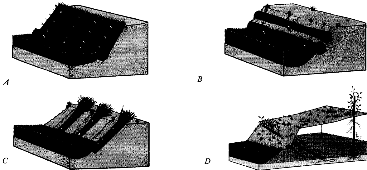
Figure 2A-D. Streambank bioengineering uses nonrooted hardwood cuttings of cottonwood and willows in a variety of treatments: A) brush mattress, B) willow wattle, C) vertical bundle, and D) pole cuttings.
