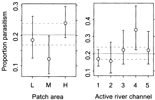
FIG. 1. Mean proportion of brood parasitism with 95% confidence intervals within each category of patch area and each category of active river channel. Overall estimated frequency of brood parasitism (0.202; horizontal line) and confidence intervals (dashed line) are displayed for comparison. Abbreviations for the predictors and values for each category are provided in Table 1.
